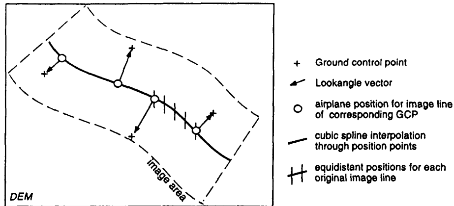
Figure 3: The ground control points based flightpath reconstruction procedure
