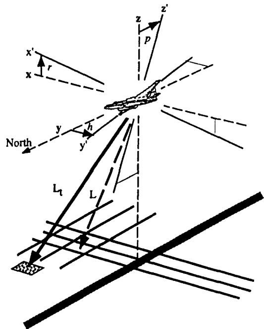
Figure 1: Transformation of the theoretical look angle vector L to the effective look angle vector L_t . r , p and h denote roll, pitch and true heading angles respectively [modified after Meyer, 1994].
